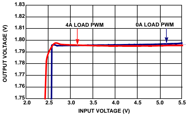
FIGURE 13. OUTPUT VOLTAGE REGULATION vs V_{IN} (PWM V_{OUT} = 1.8\text{V} )
