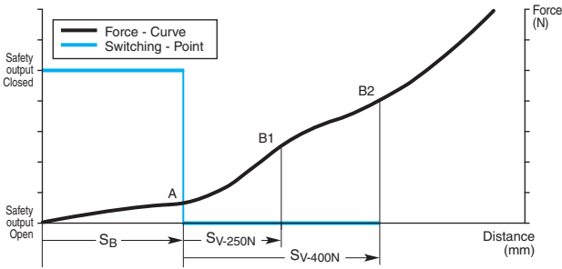
SGE-125: Characteristic Values for Test Speed v = 10 \text{ mm/s}
