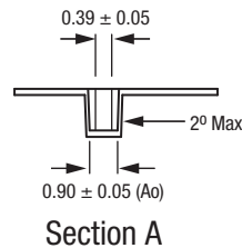
Figure 9. SC-79 Tape and Reel Dimensions
