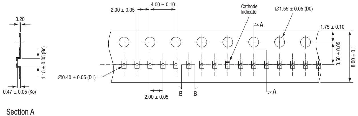
Figure 12. SOD-882 Package Dimension Drawing
