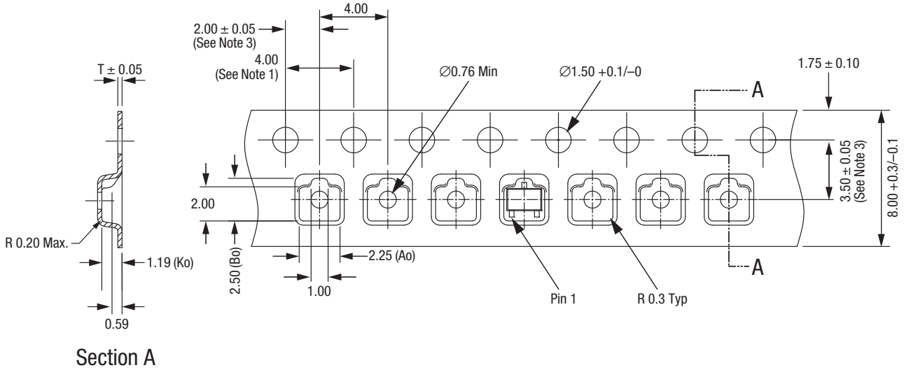
Figure 6. SC-70 Package Dimension Drawing
