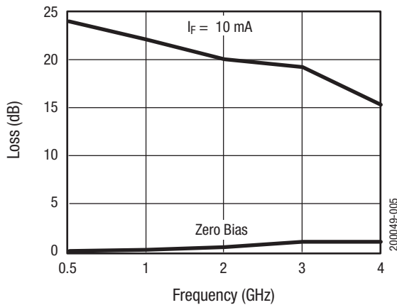
Figure 5. SMP1322-017 Typical SPST Switch Performance
