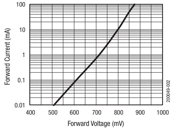
Figure 2. DC Characteristics
